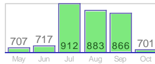
#Overlapping Keywords (701)
