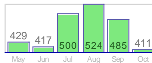
#Overlapping Keywords (411)
