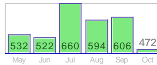
#Overlapping Keywords (472)
