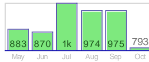
#Overlapping Keywords (793)
