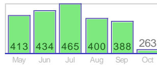
#Overlapping Keywords (263)
