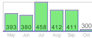
#Overlapping Keywords (300)
