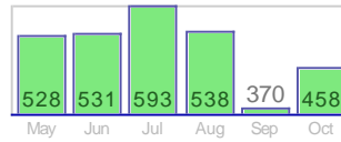
#Overlapping Keywords (458)
